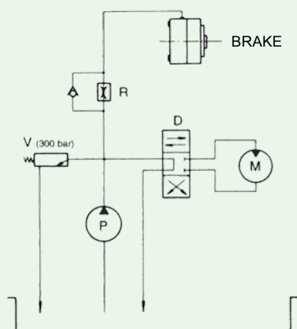
Open circuit hydraulic diagram
